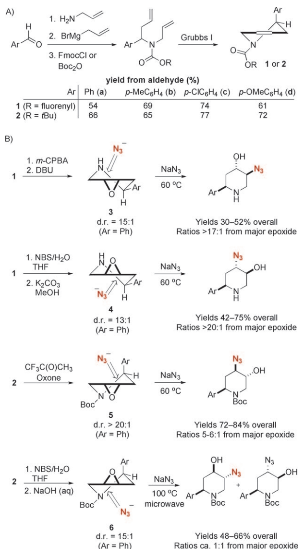
Scheme 3. Preparation of scaffold precursors by A) tetrahydropiperidine synthesis and B) stereoselective epoxidation reactions and allylic strain control of regiochemistry of epoxide ring opening (general reaction conditions for azidation: NaN_3 , NH_4Cl , MeOH/H_2O (3:1), 60^\circ C ). Boc = tert -butoxycarbonyl, Fmoc = 9-fluorenylmethyloxycarbonyl, m CPBA = meta -chloroperbenzoic acid, NBS = N -bromosuccinimide, THF = tetrahydrofuran.
