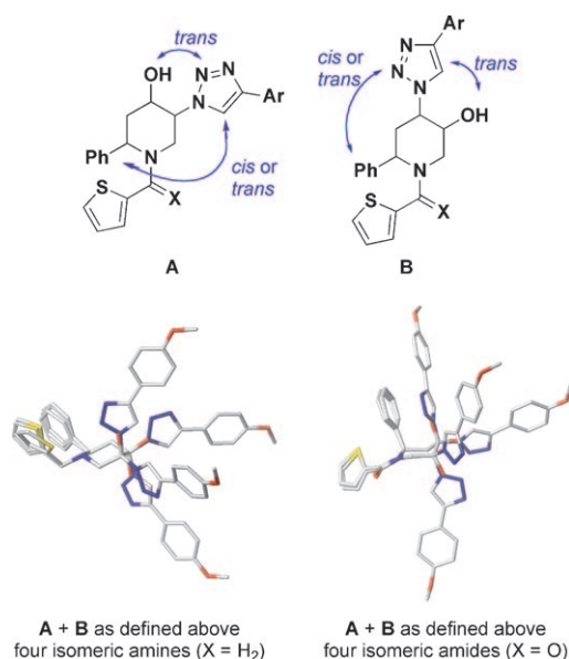
Scheme 2. Conformational diversity of targeted library containing sp^3 and sp^2 hybridized N-substituted versions of scaffolds A and B . In all, eight idealized conformers (four amines and four amides, all piperidines as chairlike conformation) are shown in the two overlays. Details, including the calculations of individual structures, are provided in the Supporting Information.
